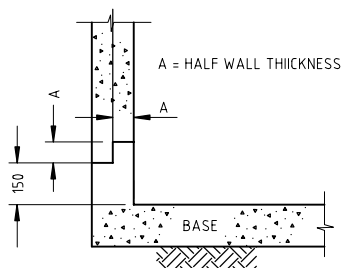
CONSTRUCTION JOINT
